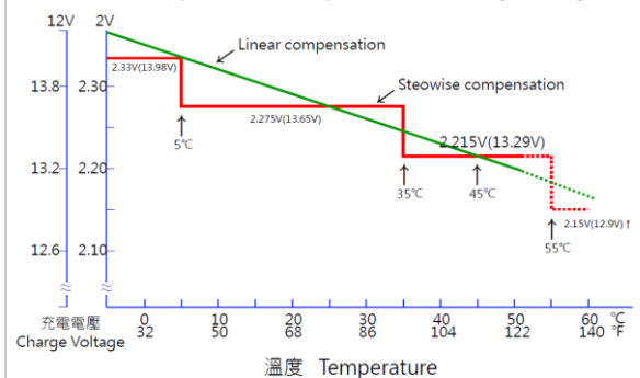
溫度與充電電壓關係 Relationship Between Temperature and Charge Voltage
